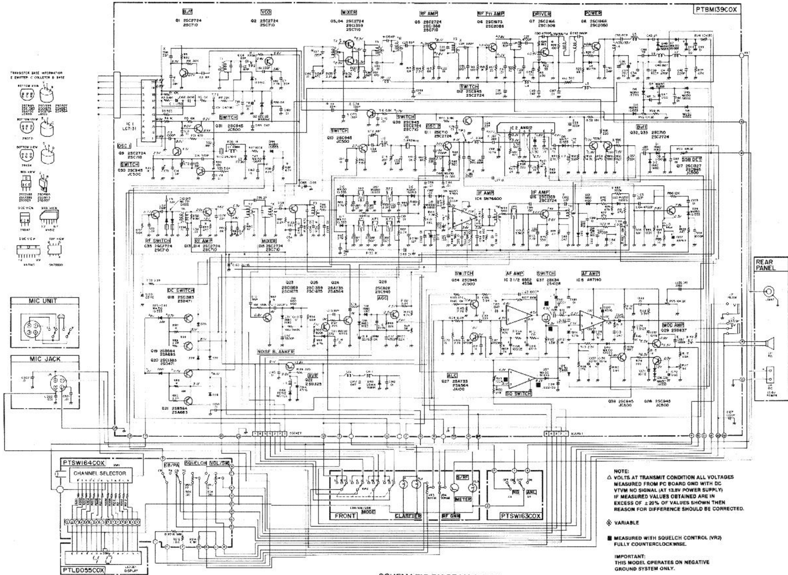
SCHEMATIC DIAGRAM 3-5826A
